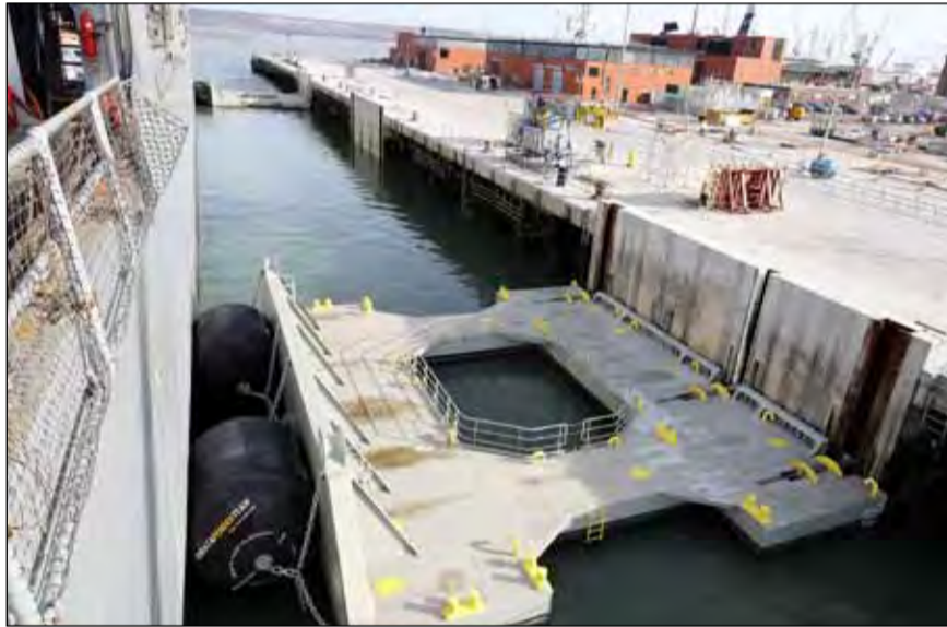
● The new fender spacer units are tested at Princess Royal Jetty Picture: LPhot Iggy Roberts
